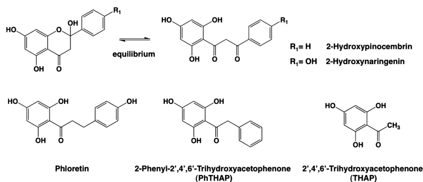
Figure 1. Substrates used in this study.
