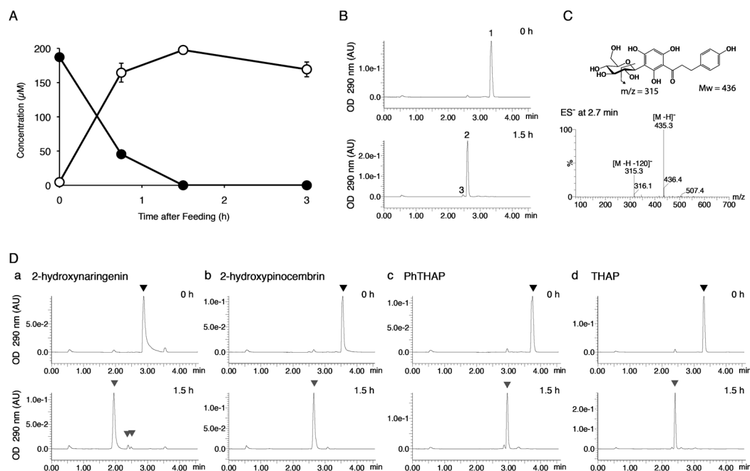
Figure 2. Production of C-glycosides of flavonoids and related compounds by Escherichia coli expressing buckwheat C-glucosyltransferase (FeCGTa). A. Changes in the culture media after the addition of phloretin (final, 200 \mu\text{M} ). Filled circles and open circles represent the concentrations of phloretin and nothofagin, respectively. B. HPLC profiles of the culture media at 0 and 1.5 h after the addition of phloretin. Peak identifications: 1, phloretin; 2, nothofagin; 3, uncharacterized metabolite of nothofagin. C. Mass spectrum of peak 2 (2.7 min) from B. D. HPLC profiles of culture media at 0 and 1.5 h after the addition of substrates. a: 2-Hydroxynaringenin; b: 2-hydroxypinocembrin; c: 2-phenyl-2',4',6'-trihydroxyacetophenone (PhTHAP); and d: 2',4',6'-trihydroxyacetophenone (THAP). Black and gray arrowheads indicate the peaks of administered substrates and their C-glycosides, respectively. The small peaks in "a" are the dehydrated products of C-glycoside (vitexin and isovitexin).
