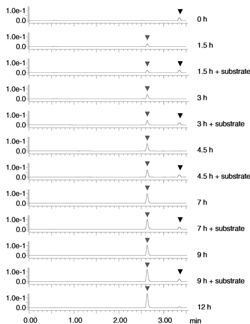
Figure 4. Production of C-glucoside by Escherichia coli expressing buckwheat C-glucosyltransferase (FeCGTa), with repeated addition of the substrate. Phloretin ( 200\ \mu\text{M} ) was added to the culture of E. coli expressing FeCGTa in 1.5–2 h intervals, as indicated in the figure, and analyzed by HPLC as described in the “Materials and methods” section. Black and gray arrowheads indicate the peaks of added phloretin and produced nothofagin, respectively.
