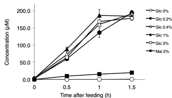
Figure 3. Effect of glucose concentration on C-glucoside production by Escherichia coli expressing buckwheat C-glucosyltransferase (FeCGTa). Glc, glucose; Mal, maltose.
