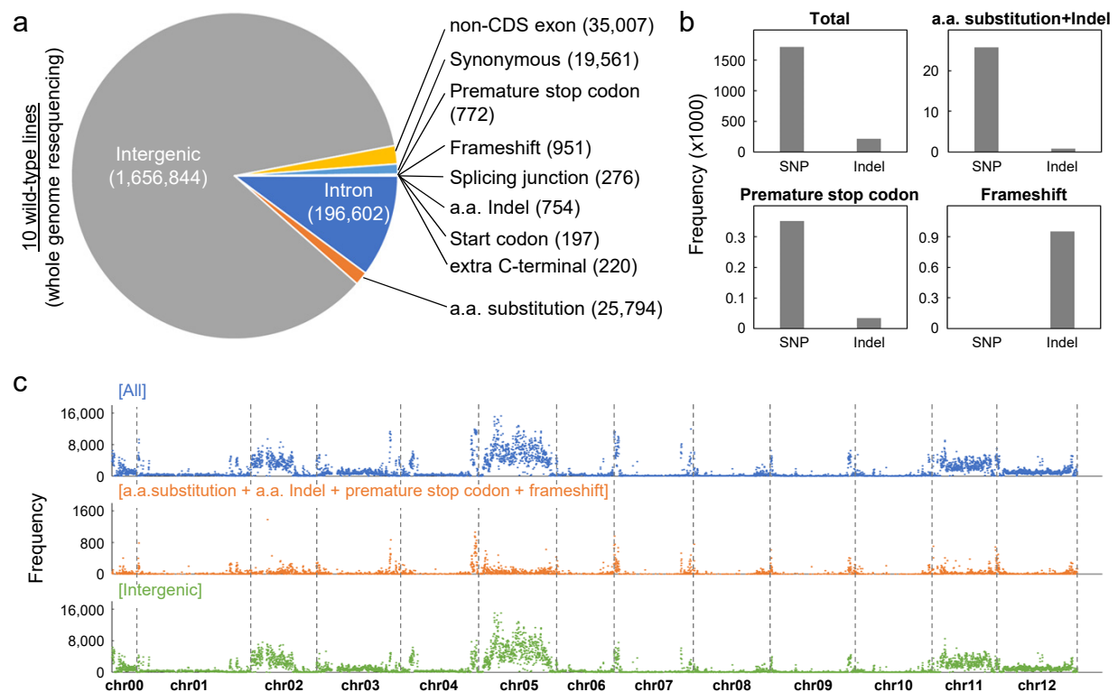
Supplementary Figure S2. Statistic summary of DNA variants identified in 95 ‘Micro-Tom’ mutants. (a) A diagram showing the frequency of mutation type in the DNA variant dataset of 10 wild types. (b) Frequencies of single nucleotide polymorphisms (SNPs) and Indels in each mutation type in the DNA variant dataset of 10 wild types. (c) Genome-wide distribution and frequency of DNA variants (natural polymorphisms) in 10 wild-type ‘Micro-Tom’ lines based on the tomato genome reference Heinz1706 SL3.0/ITAG3.10.
